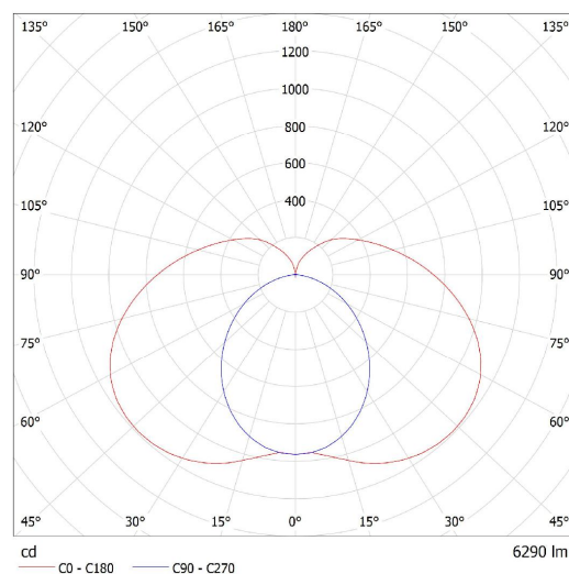
Lucis ZT.AU1.L12.1500.X AULA LED / LDC (Polar)
